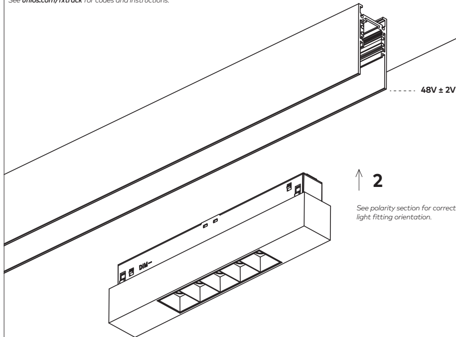
Track Fixture Positioning
